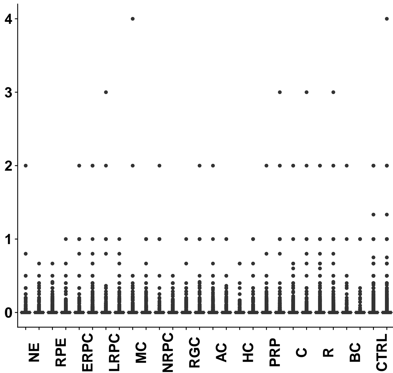
Tef_1_mean
