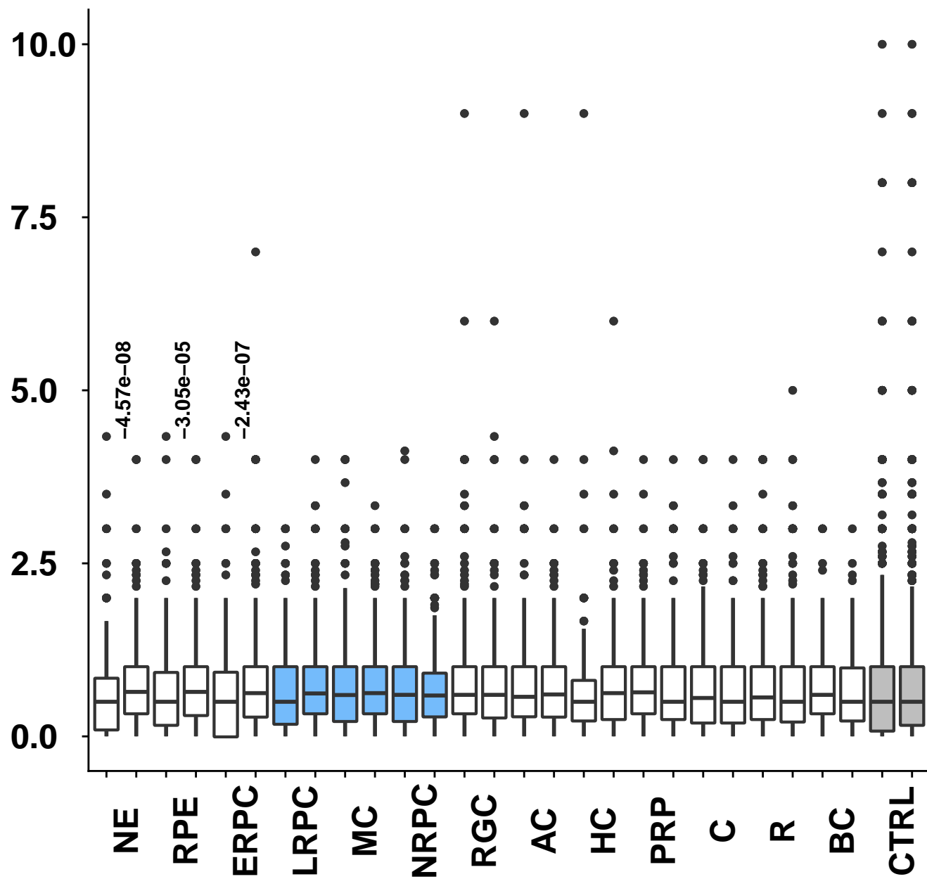
Tcf4_2_mean
