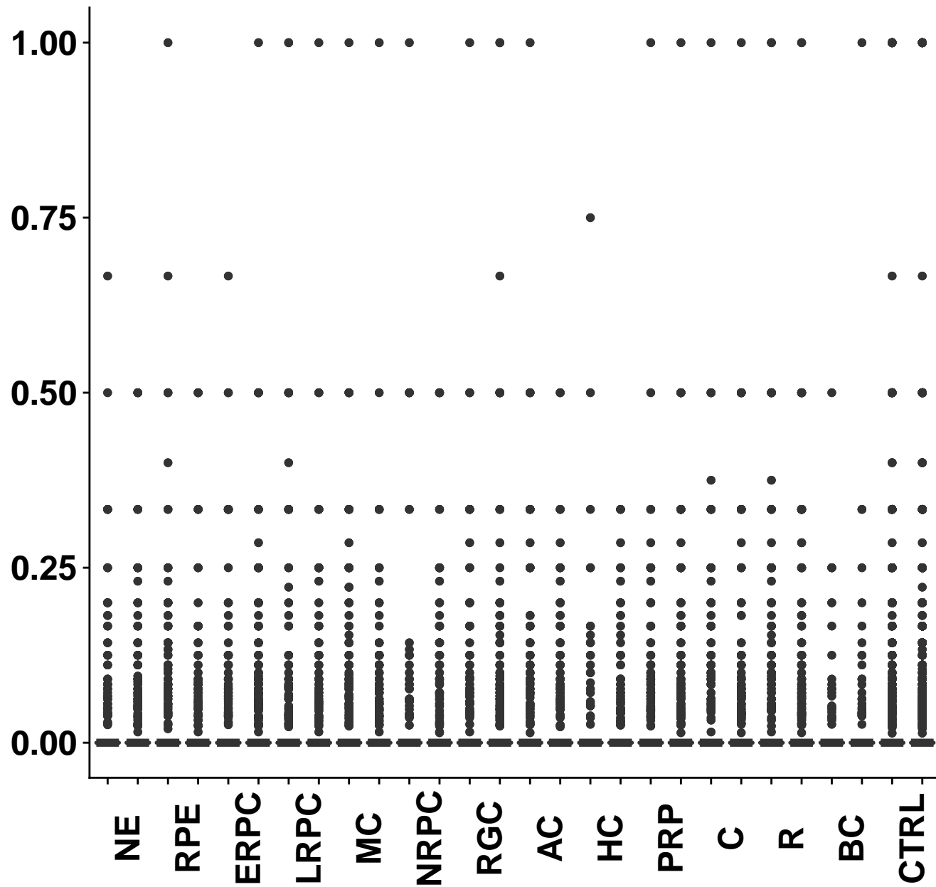
Six6_1_mean
