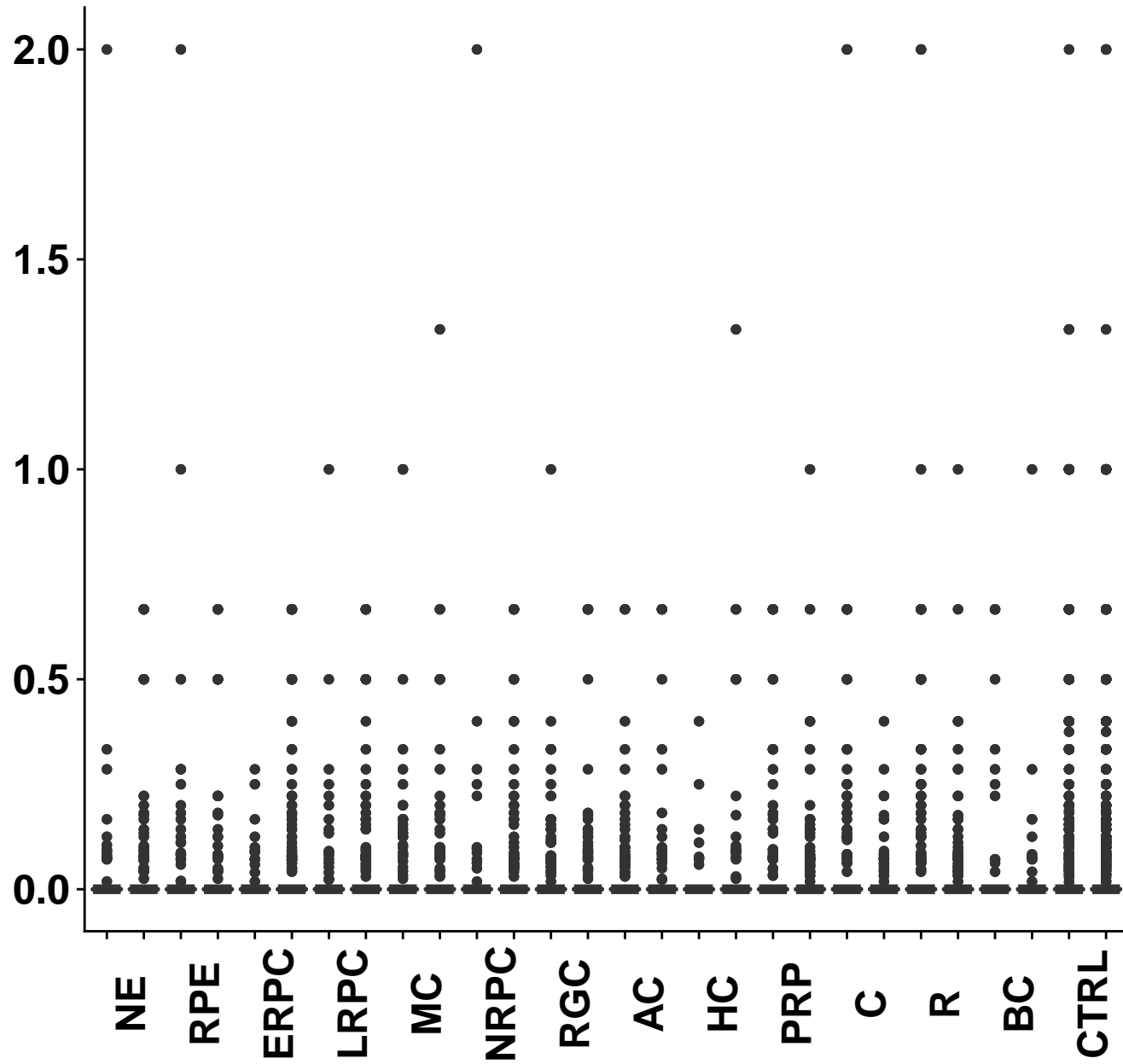
Mafg_2_mean
